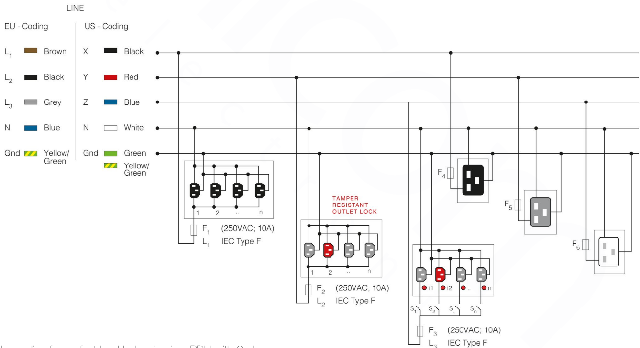
Color coding for perfect load balancing in a PDU with 3 phases
