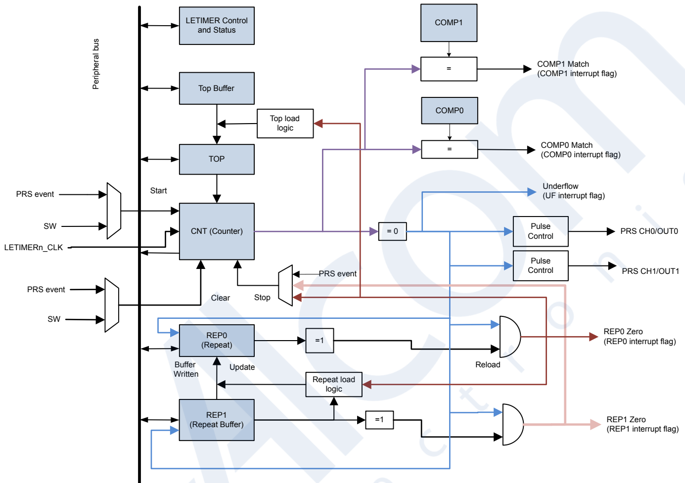
Figure 18.1. LETIMER Overview
