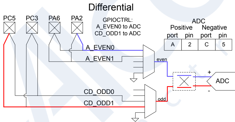
Figure 23.15. Differential Port/Pin Selection without Swap
