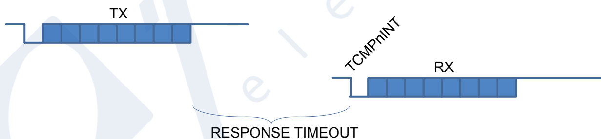
Figure 20.26. USART Response Timeout
