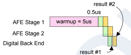
Figure 23.5. High-Speed Mode ADC Pipeline
