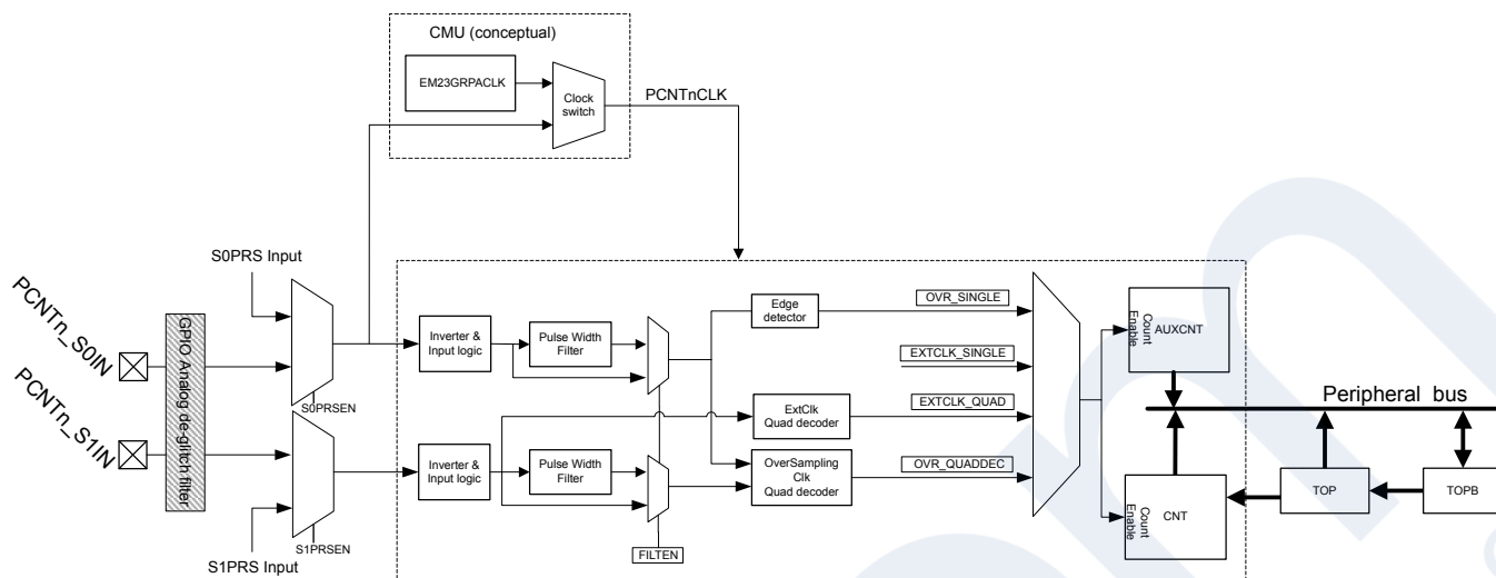
Figure 27.1. PCNT Overview
