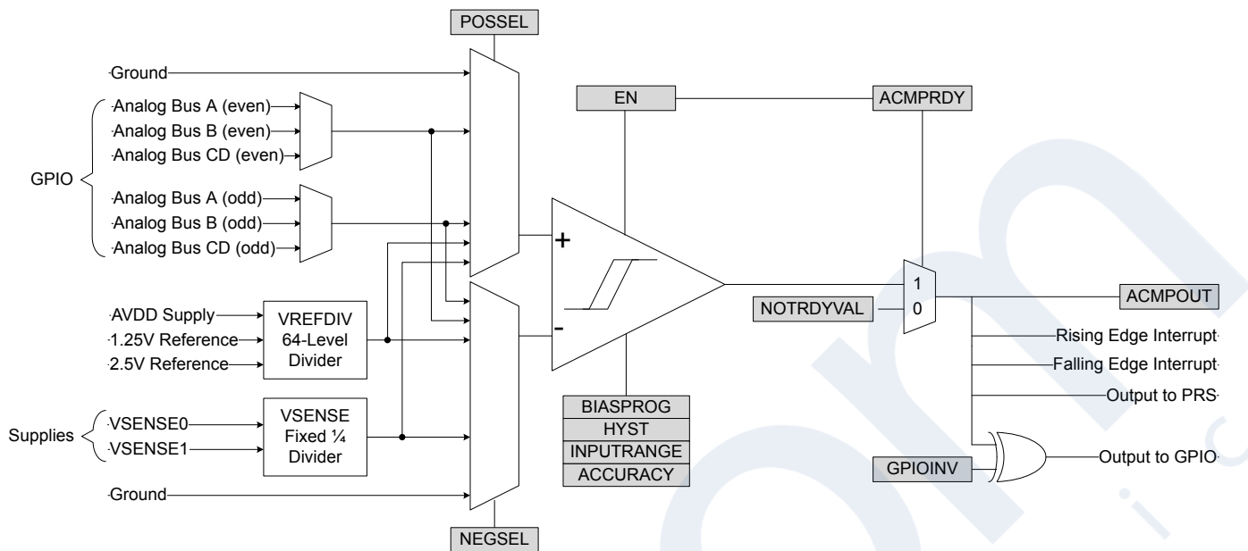
Figure 29.1. ACMP Overview
