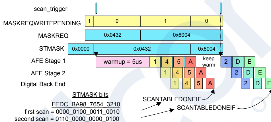
Figure 23.18. MASKREQ Updates
