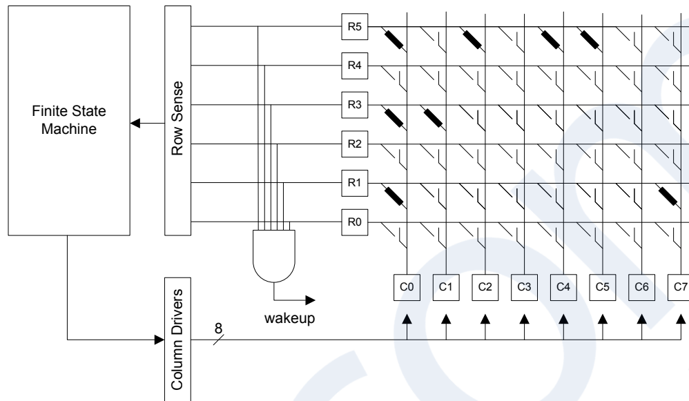
Figure 30.1. KEYSCAN Overview
