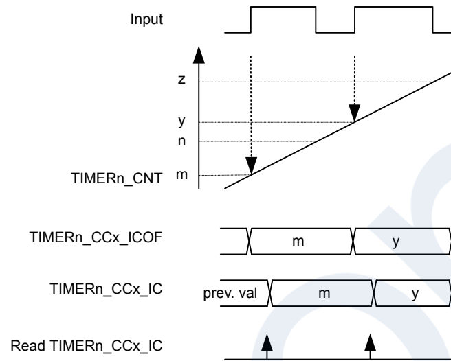
Figure 19.12. TIMER Input Capture
