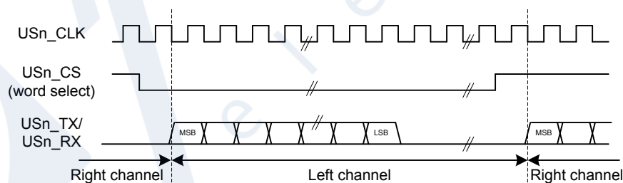
Figure 20.21. USART Standard I2S Waveform (Reduced Accuracy)
