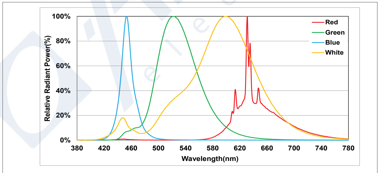
Figure 2: Typical Color Spectrum (RGBW)
