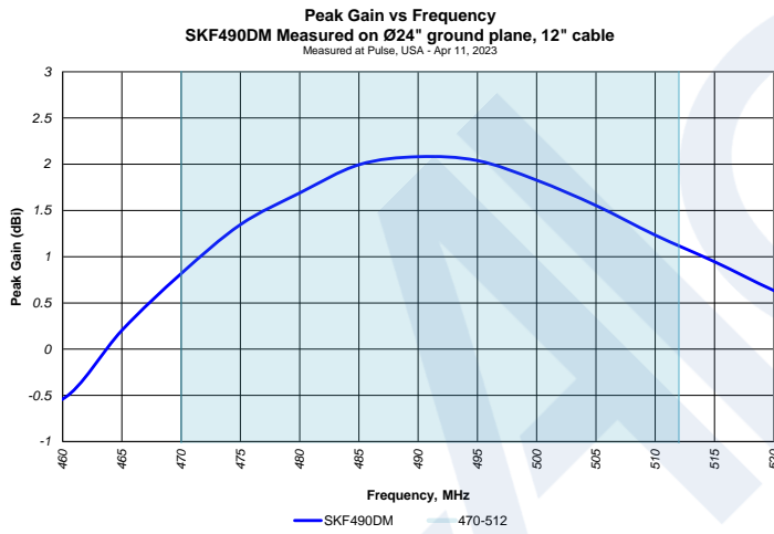
antenna sample measured on \varnothing 24" (609.6mm) ground plane
