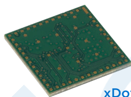
xDot LGA Family Footprint
