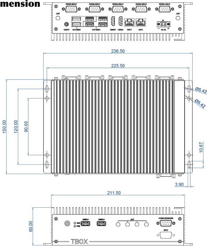
DIMENSIONAL DRAWING:TBOX-2E15
