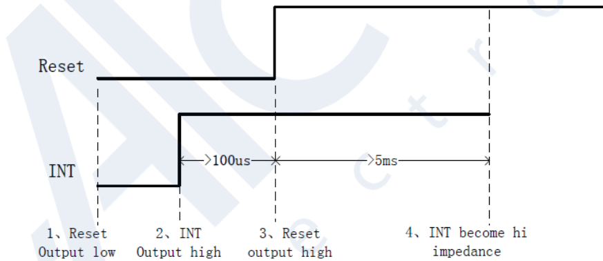
Fig.8(a) Timing of setting slave address
