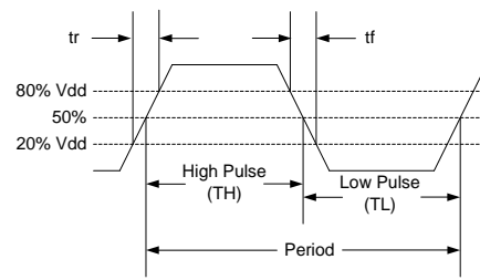
Figure 3. Waveform [7]
