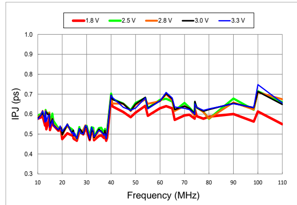
Figure 12. RMS Integrated Phase Jitter Random (900 kHz to 20 MHz) vs Frequency [10]
