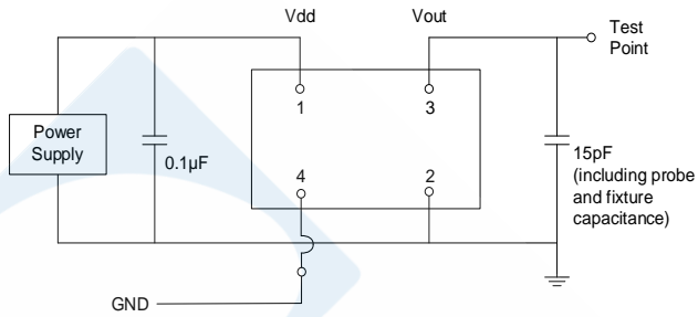
Figure 2. Test Circuit [7]
