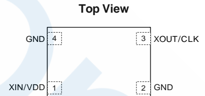
Figure 1. Pin Assignments
