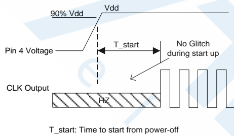
Figure 4. Startup Timing [8]
