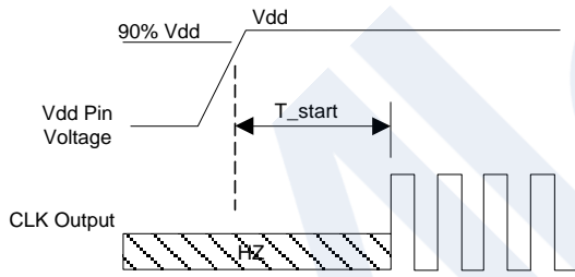
Figure 11. Startup Timing
