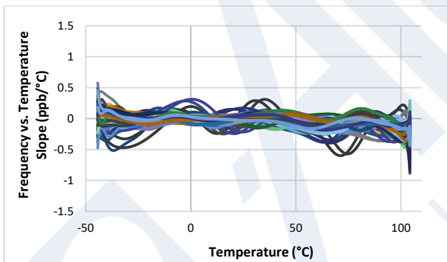
Figure 18. Freq. vs. Temp. Slope ( \Delta F/\Delta T )
