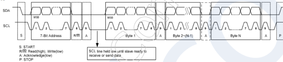
Figure 4-1 I2C Waveform
