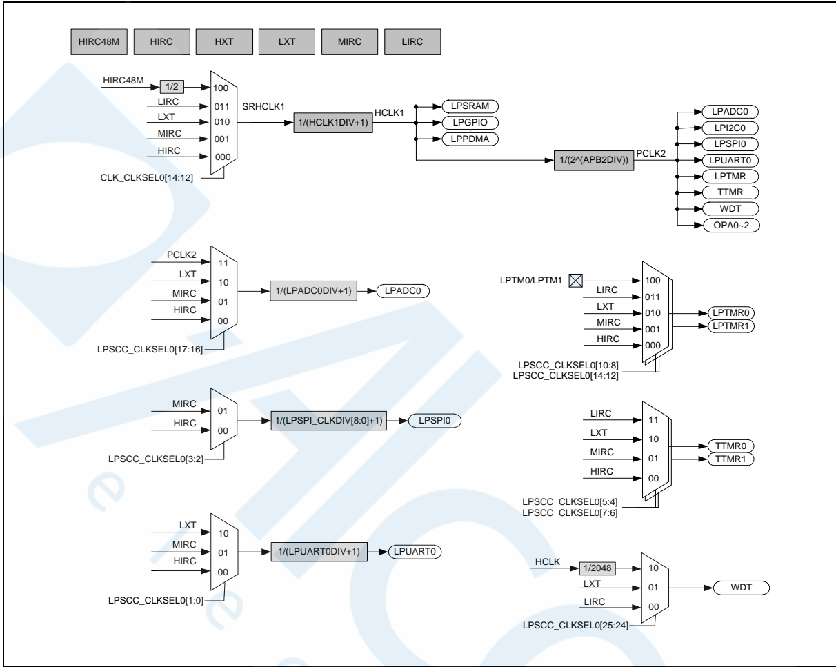
Figure 6.3-2 Low Power Domain Clock Generator Global View Diagram
