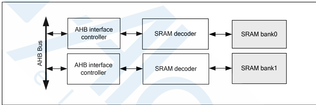
Figure 6.2-9 SRAM Block Diagram
