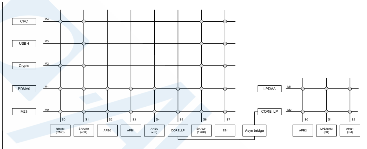
Figure 6.2-13 NuMicro M2L31 Bus Matrix Diagram
