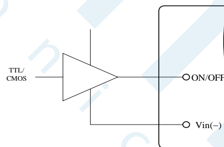
Figure 4. Direct Logic Drive
