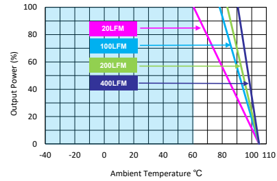
MTQZ75-72S12, MTQZ75-72S15 Derating Curve with Heatsink
