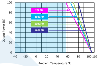
MTQZ75-72S12, MTQZ75-72S15 Derating Curve without Heatsink
