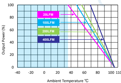
MTQZ75-72S05, MTQZ75-110S05 Derating Curve without Heatsink
