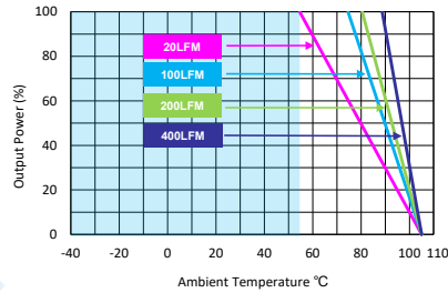
MTQZ75-110S12, MTQZ75-110S15, MTQZ75-72S24 Derating Curve with Heatsink
