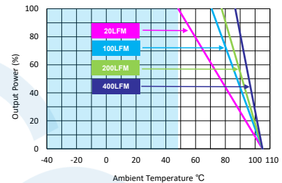
MTQZ75-110S24 Derating Curve with Heatsink
