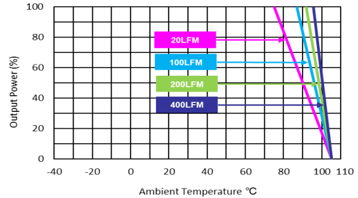
MTQZ50-72S12, MTQZ50-72S15, MTQZ50-110S15 Derating Curve with Heatsink
