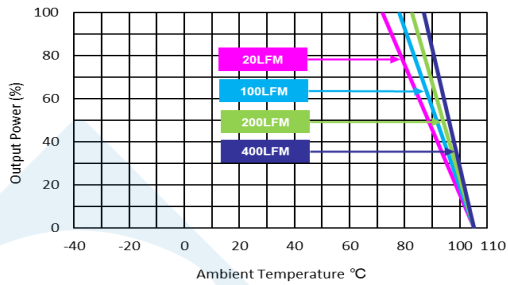
MTQZ50-72S12, MTQZ50-72S15, MTQZ50-110S15 Derating Curve without Heatsink
