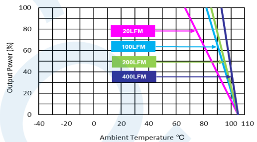
MTQZ50-72S05, MTQZ50-110S05 Derating Curve with Heatsink
