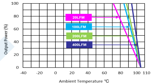
MTQZ50-72S24, MTQZ50-110S12, MTQZ50-110S24 Derating Curve with Heatsink
