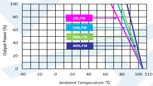
MTQZ50-72S24, MTQZ50-110S12, MTQZ50-110S24 Derating Curve without Heatsink
