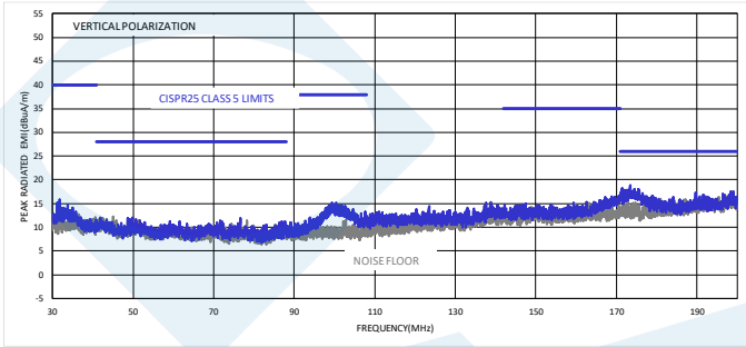
CISPR25 Class 5 Peak Radiated Emissions Vertical, 30MHz to 200MHz
