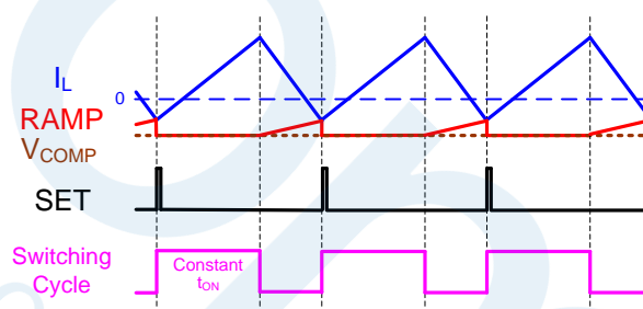
Figure 18: FCCM under Light-Load Conditions
