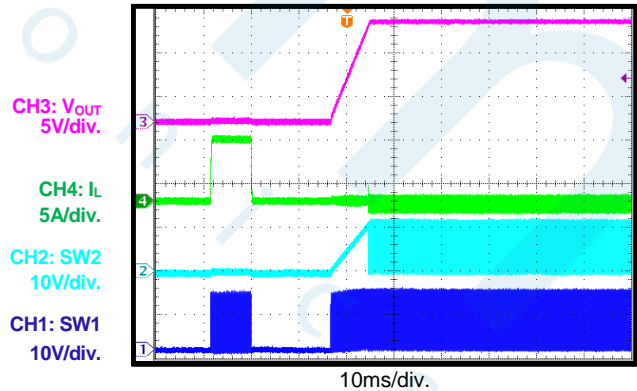
SCP Recovery
