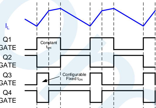
Figure 8: Buck-Boost Mode in Normal FCCM ( V_{IN} > V_{OUT} )
