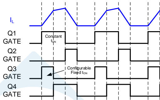
Figure 9: Buck-Boost Mode in Normal DCM ( V_{IN} > V_{OUT} )
