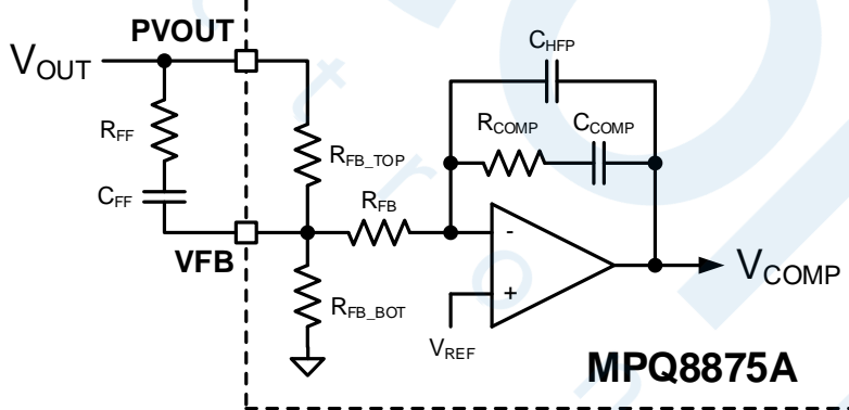
Figure 26: Control Loop Compensation Network
