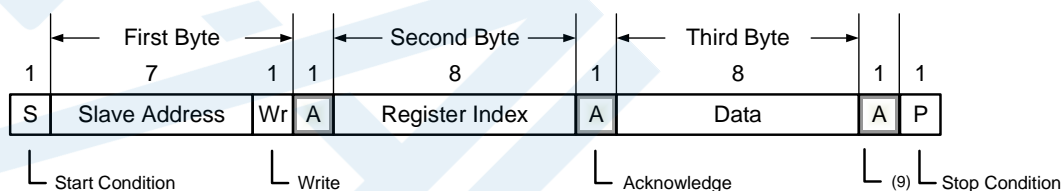
Figure 24: Write Sequence (9)
