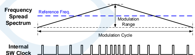
Figure 16: Frequency Spread Spectrum
