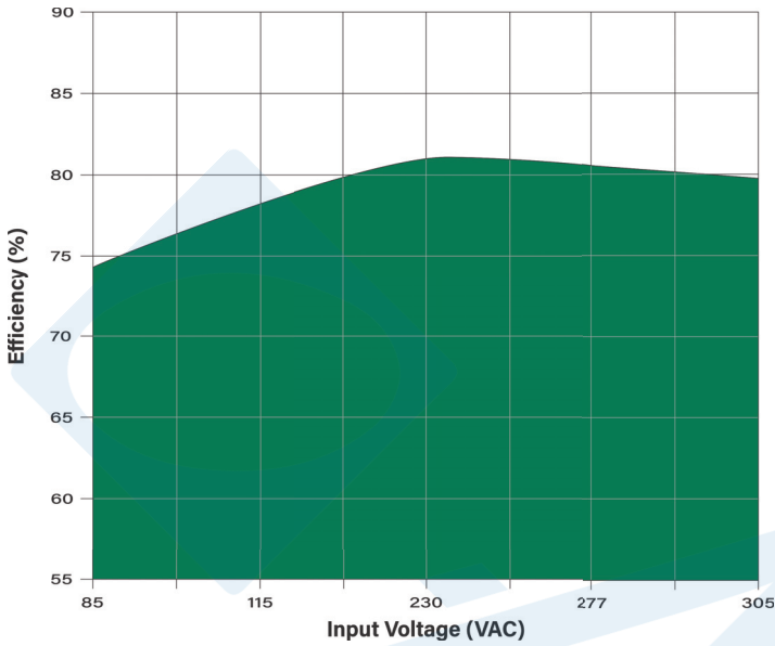
Efficiency vs Input Voltage: MPL-10S-24SEUP
