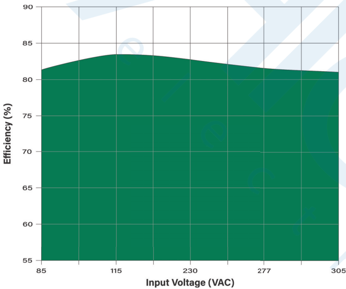
Efficiency vs Input Voltage: MPL-10S-24SEUP
