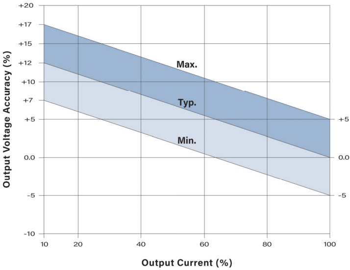
MIG215L-1509HI: +15V Output
