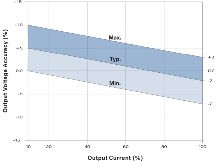
MSC224L-1509HI: -9V Output
