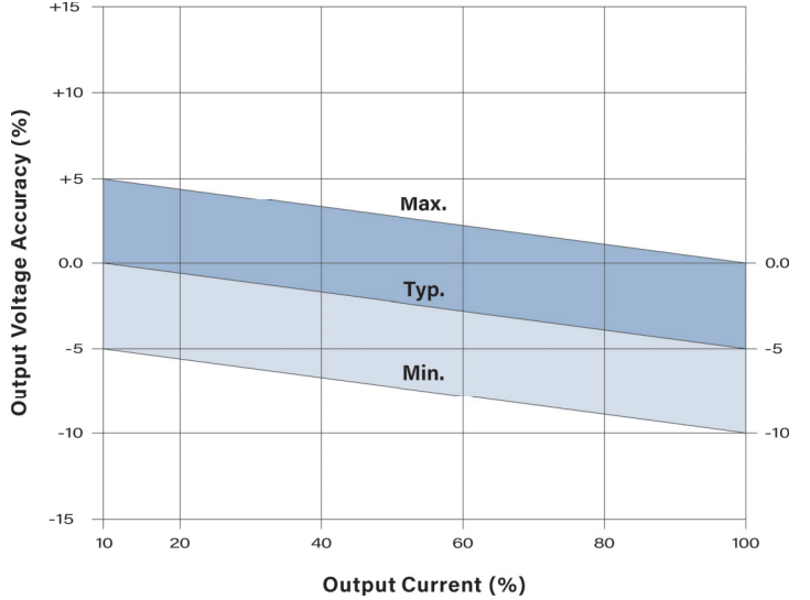
MSC224L-1509HI: -9V Output
