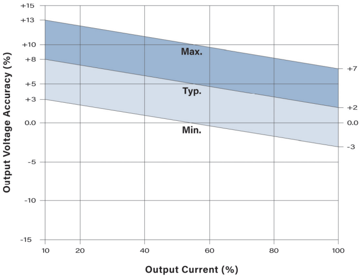
MIG224L-1509HI: +15V Output
