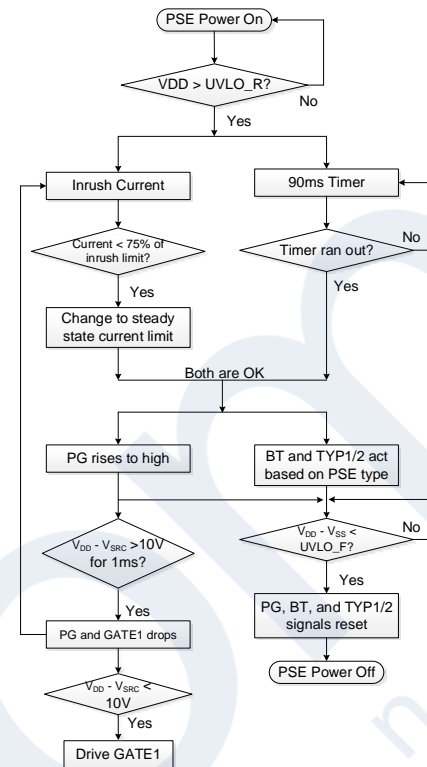
Figure 3: PG Logic
