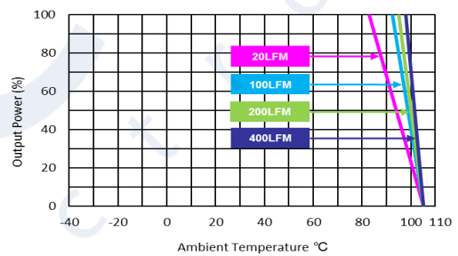
MKZI10-110S05 Derating Curve with Heatsink
