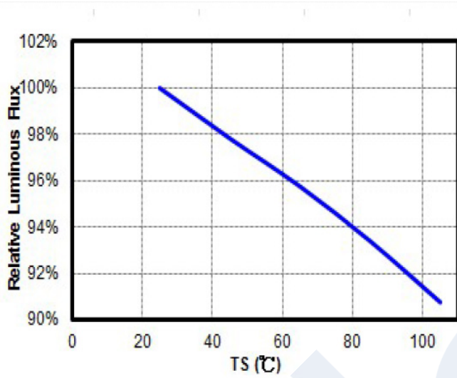
Solder Point Temp. vs. Relative Luminous Flux
