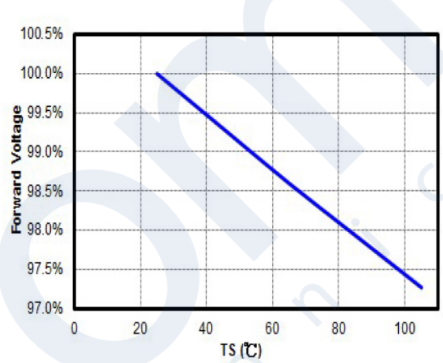
Solder Point Temp. vs. Relative Forward Voltage
