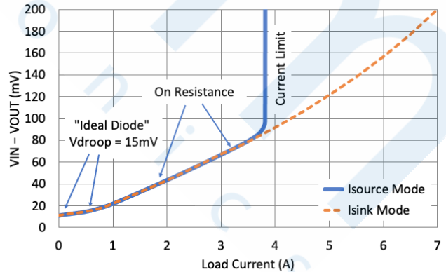
"Ideal Diode" Vdroop vs. Load Current ( V_{IN} \geq 5\text{V} , enabled, R_{ISET} = 14.7\text{k}\Omega )
