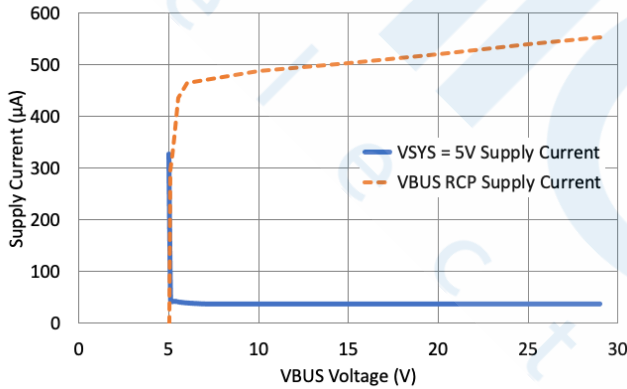
RCP Supply Current in Isource Mode ( V_{SYS} = 5\text{V} , enabled, V_{BUS} lifted)
