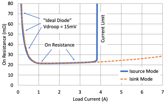
On Resistance vs. Load Current ( V_{IN} \geq 5\text{V} , enabled, R_{ISET} = 14.7\text{k}\Omega )
