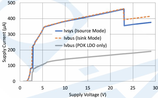
Supply Current vs. Supply Voltage (enabled, no load)
