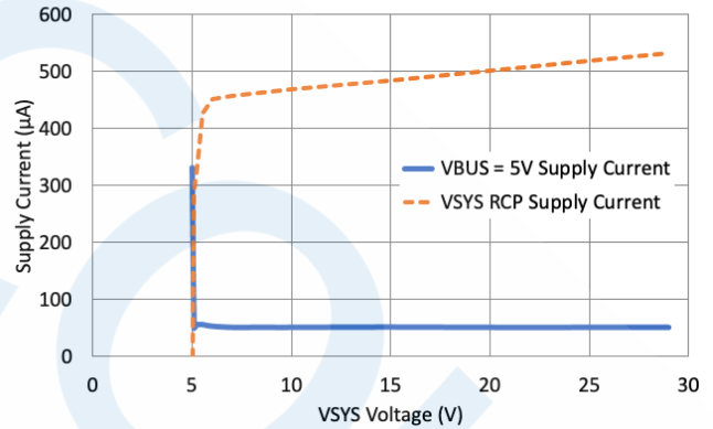
RCP Supply Current in Isink Mode ( V_{BUS} = 5\text{V} , enabled, V_{SYS} lifted)
