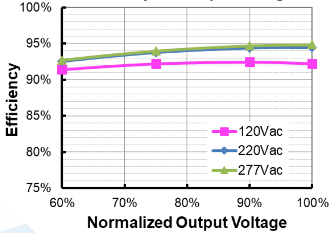
EUM-680S240Mx ( I_o=2400mA ) Efficiency vs. Output Voltage
