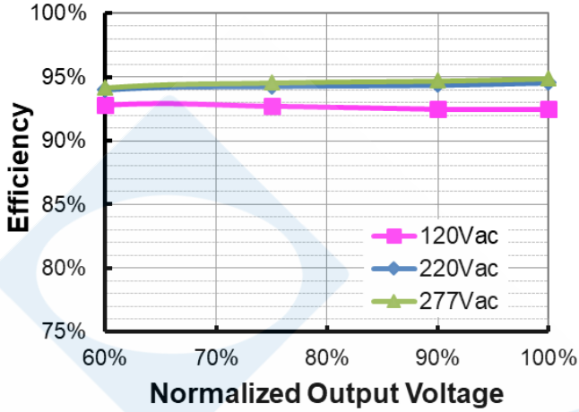
EUM-680S240Mx ( I_o=1800mA ) Efficiency vs. Output Voltage
