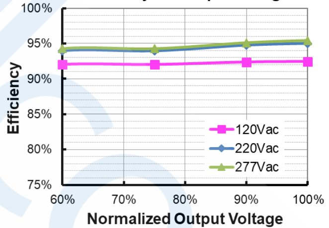
EUM-680S350Mx ( I_o=3500mA ) Efficiency vs. Output Voltage
