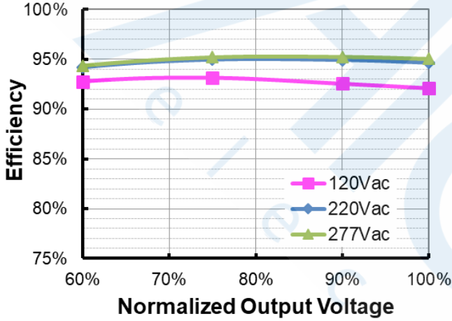
EUM-680S350Mx ( I_o=2600mA ) Efficiency vs. Output Voltage
