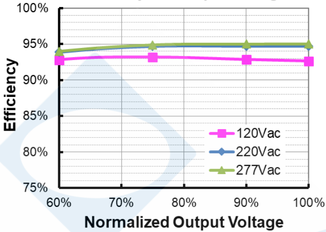
EUM-680S840Mx (Io=6300mA) Efficiency vs. Output Voltage
