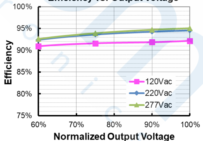
EUM-680S560Mx ( I_o=5600mA ) Efficiency vs. Output Voltage
