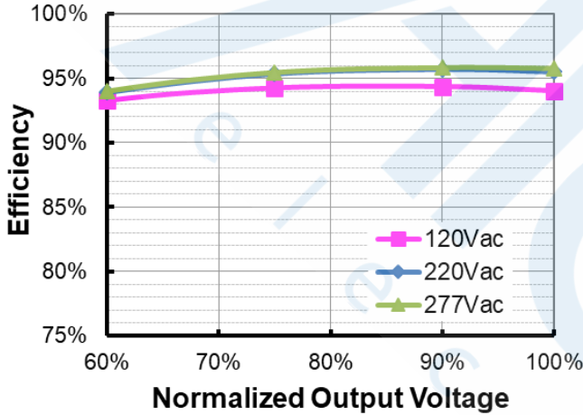
EUM-680S15AMx (Io=12600mA) Efficiency vs. Output Voltage
