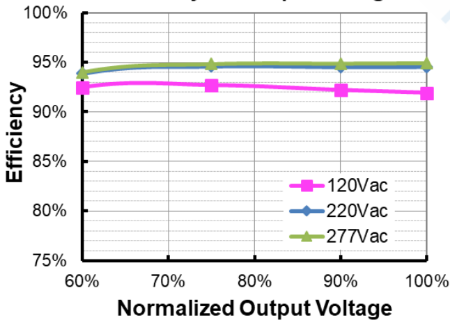
EUM-680S560Mx ( I_o=4200mA ) Efficiency vs. Output Voltage
