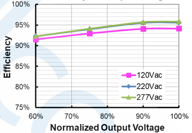
EUM-680S15AMx (Io=15000mA) Efficiency vs. Output Voltage
