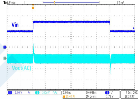
HT7727FA Line Transien
