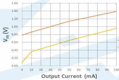
HT7730FA Start Up & Hold On
