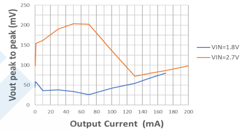
HT7730FA Ripple @L=10μH Cout=10μF
