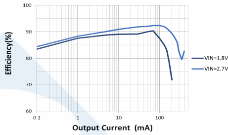
HT7730FA Efficiency
