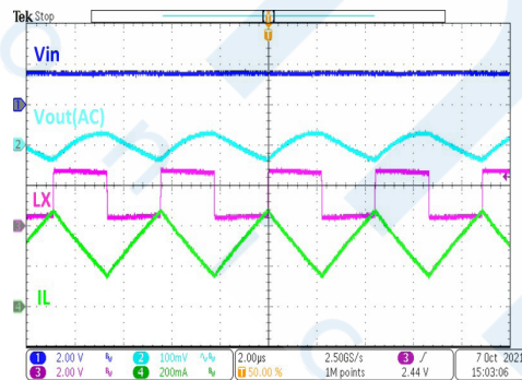
HT7727FA Operation ( I_{OUT}=150mA )
