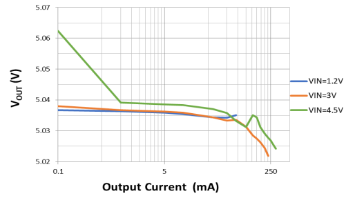
HT7750FA Load regulation
