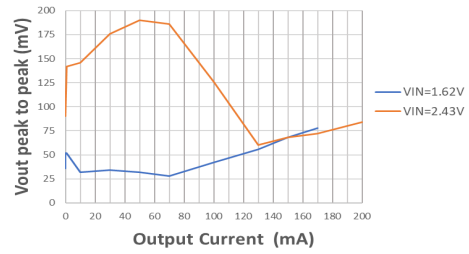
HT7727FA Ripple @L=10μH Cout=10μF
