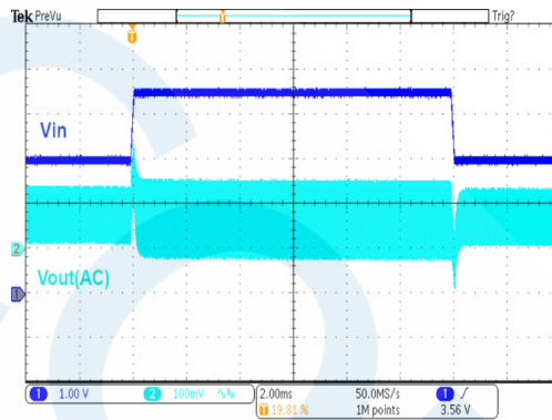
HT7750FA Line Transient ( V_{IN}=3V\sim 4.5V , I_{OUT}=200mA )
