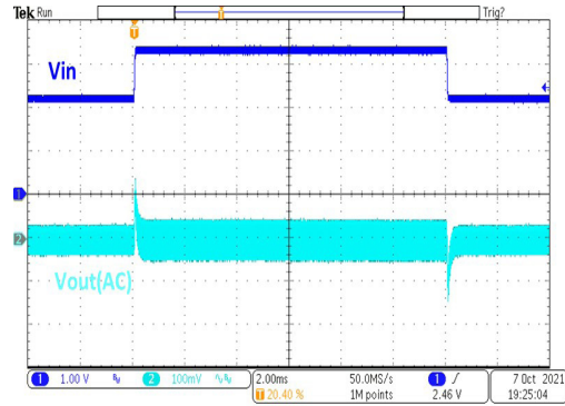
HT7737FA Line Transient ( V_{IN}=2.22V\sim 3.33V , I_{OUT}=150mA )
