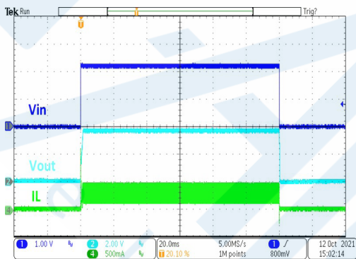
HT7737FA Power On/Off ( V_{IN}=2.22V , I_{OUT}=150mA )
