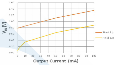
HT7727FA Start Up & Hold On
