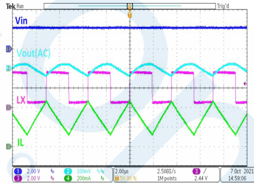
HT7737FA Operation ( I_{OUT}=150mA )
