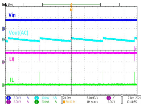
HT7727FA Operation ( I_{OUT}=0mA )
