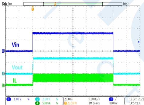
HT7727FA Power On/Off
