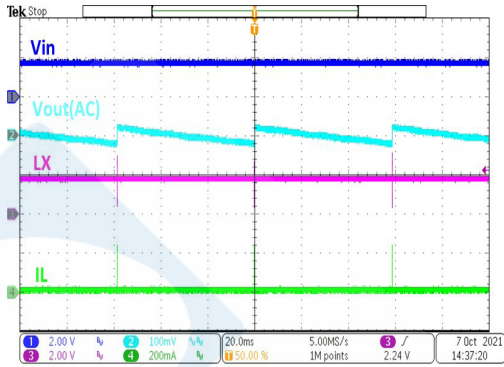
HT7730FA Operation ( I_{OUT}=0mA )
