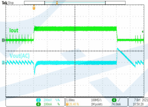
HT7727FA Load Transient
