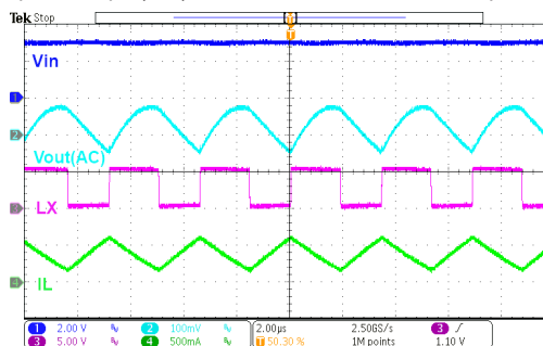
HT7750FA Operation ( I_{OUT}=200mA )
