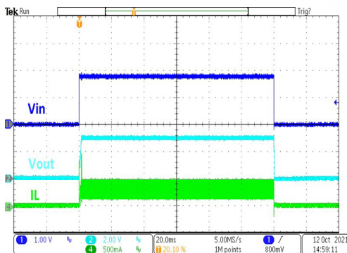
HT7730FA Power On/Off ( V_{IN}=1.8V , I_{OUT}=150mA )
