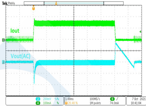
HT7737FA Load Transient ( L=10\mu H , C_{IN}=C_{OUT}=10\mu F , I_{OUT}=1mA\sim 150mA )
