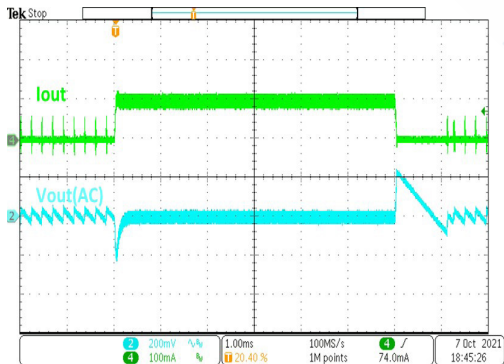
HT7733FA Load Transient ( L=10\mu H , C_{IN}=C_{OUT}=10\mu F , I_{OUT}=1mA\sim 100mA )
