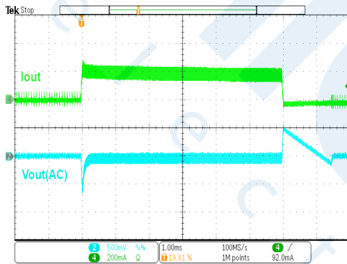
HT7750FA Load Transient ( L=10\mu H , C_{IN}=C_{OUT}=10\mu F , I_{OUT}=1mA\sim 200mA )
