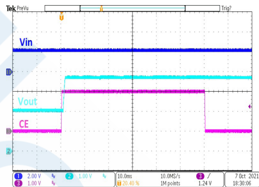
HT7737FA Chip Enable/Disable
