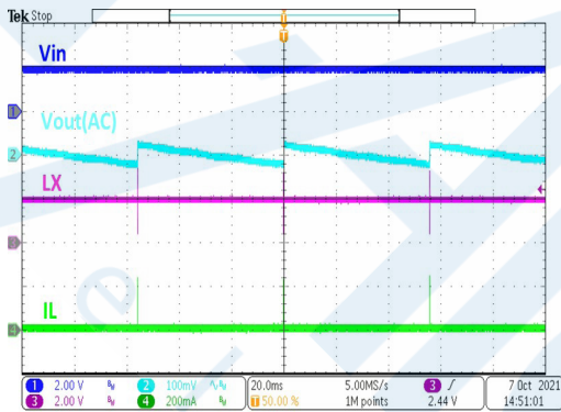
HT7733FA Operation ( I_{out}=0mA )
