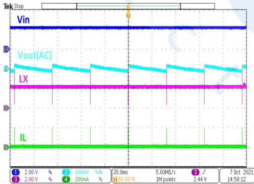
HT7737FA Operation ( I_{OUT}=0mA )
