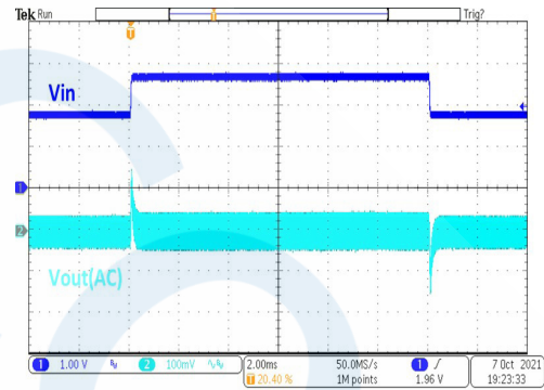
HT7730FA Line Transient ( V_{IN}=1.8V\sim 2.7V , I_{OUT}=150mA )
