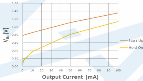
HT7750FA Start Up & Hold On
