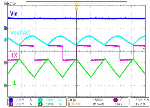
HT7730FA Operation ( I_{OUT}=150mA )
