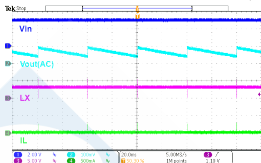
HT7750FA Operation ( I_{OUT}=0mA )
