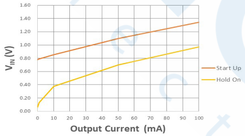
HT7733FA Start Up & Hold On
