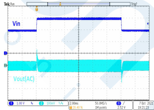
HT7733FA Line Transient ( V_{IN}=1.98V\sim 2.97V , I_{OUT}=150mA )
