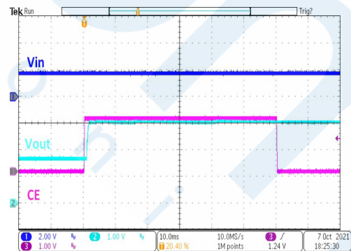
HT7730FA Chip Enable/Disable
