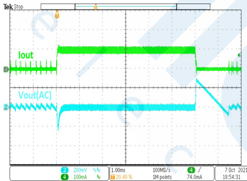
HT7730FA Load Transient ( L=10\mu H , C_{IN}=C_{OUT}=10\mu F , I_{OUT}=1mA\sim 100mA )
