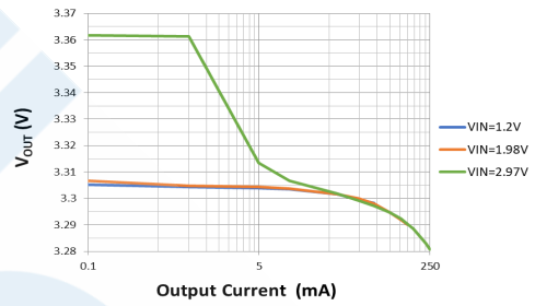
HT7733FA Load regulation
