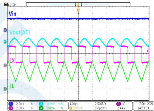
HT7733FA Operation ( I_{out}=150mA )
