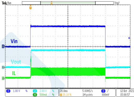
HT7733FA Power On/Off ( V_{IN}=1.98V , I_{OUT}=150mA )
