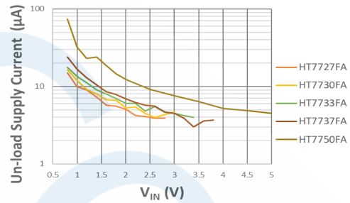
Un-load Supply Current
