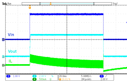
HT7750FA Power On/Off ( V_{IN}=3V , I_{OUT}=200mA )
