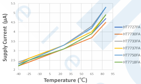
Supply Current VS Temperature
