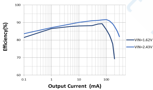
HT7727FA Efficiency
