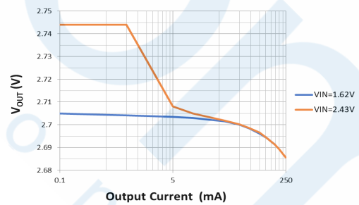
HT7727FA Load regulation
