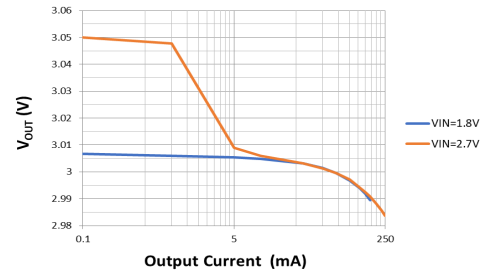
HT7730FA Load regulation
