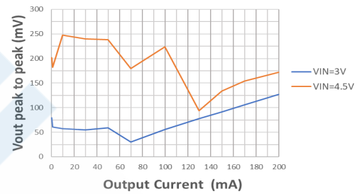
HT7750FA Ripple @L=10μH Cout=10μF
