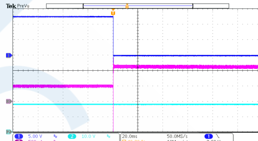
Output Short (HT7463D, I_{OUT}=500mA )
