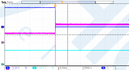
Output Short (HT7463C, I_{OUT}=500mA )
