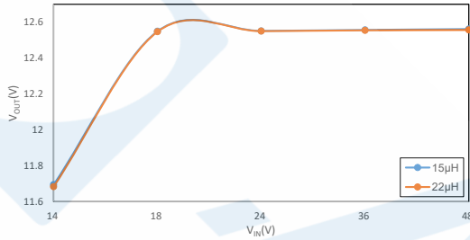
Line Regulation (HT7463C, V OUT =12.5V, I OUT =300mA)
