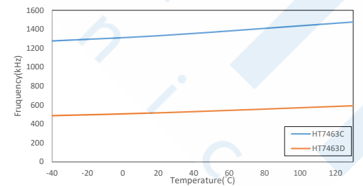
f SW vs. Temp. (HT7463C and HT7463D)
