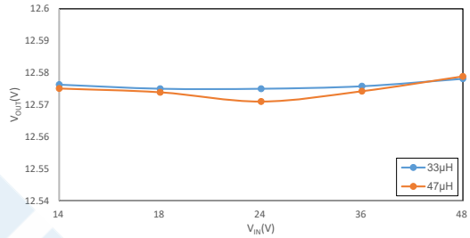
Line Regulation (HT7463D, V OUT =12.5V, I OUT =300mA)
