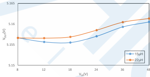
Line Regulation (HT7463C, V OUT =5V, I OUT =300mA)
