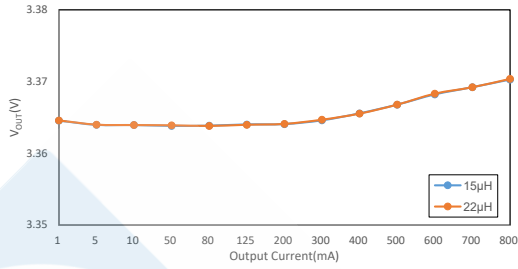
Load Regulation (HT7463C, V OUT =3.3V)
