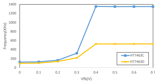
f SW vs. V FB (HT7463C and HT7463D)
