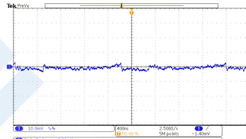
Output Ripple (HT7463D, I_{OUT}=400mA )
