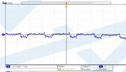
Output Ripple (HT7463C, I_{OUT}=400mA )
