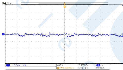
Output Ripple (HT7463C, I_{OUT}=125mA )
