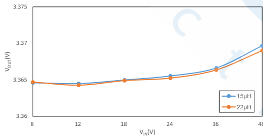
Line Regulation (HT7463C, V OUT =3.3V, I OUT =300mA)
