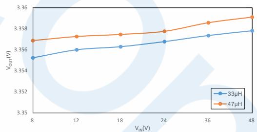
Line Regulation (HT7463D, V OUT =3.3V, I OUT =300mA)
