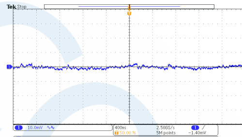
Output Ripple (HT7463D, I_{OUT}=125mA )
