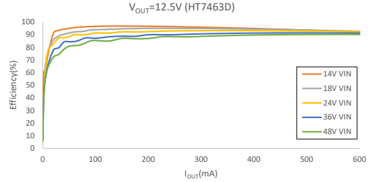
Efficiency vs. Load (HT7463D, V_{OUT}=12.5V )
