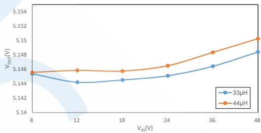
Line Regulation (HT7463D, V OUT =5V, I OUT =300mA)
