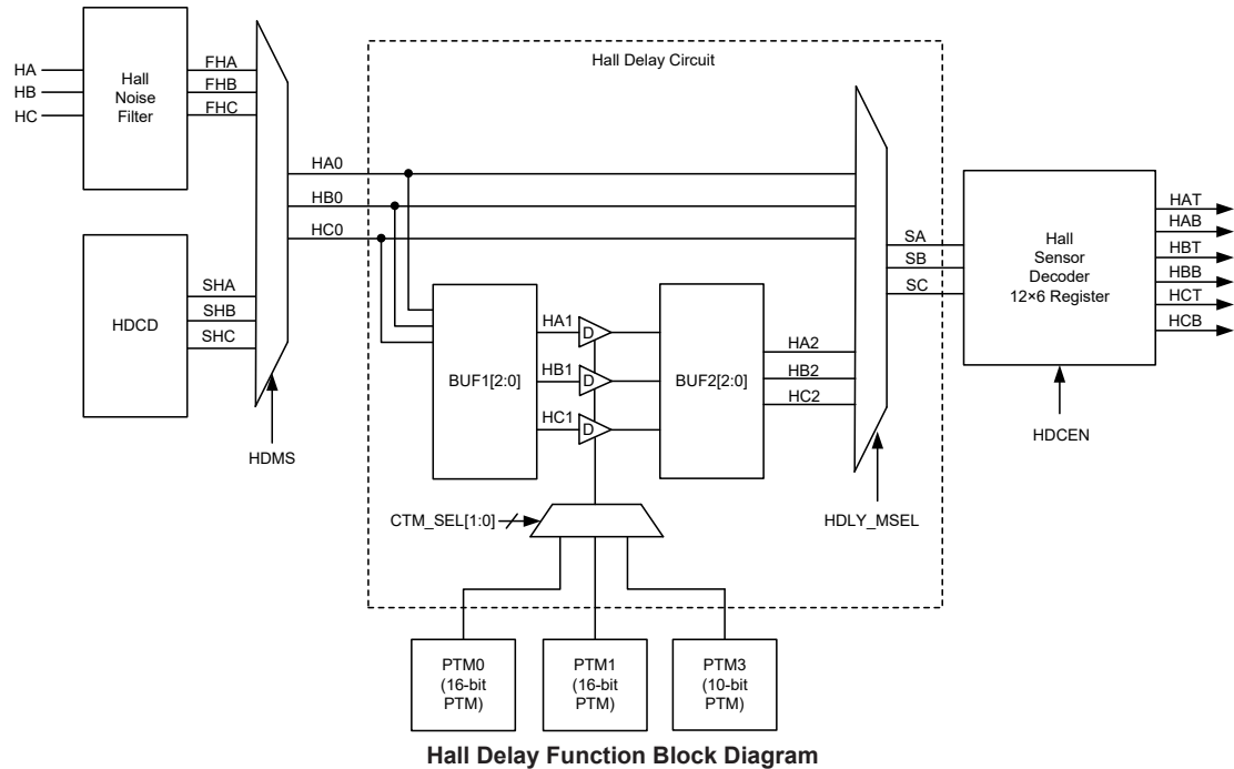
Hall Delay Function Block Diagram
