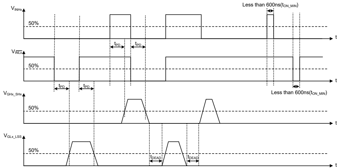
Gate-Driver Timing
