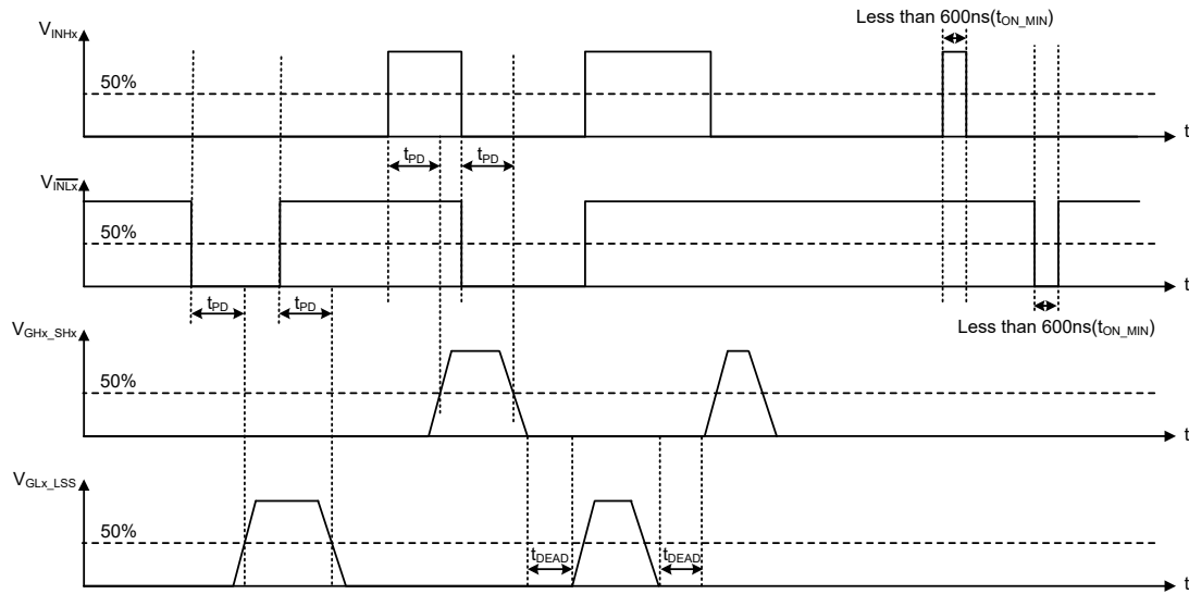
Gate-Driver Timing
