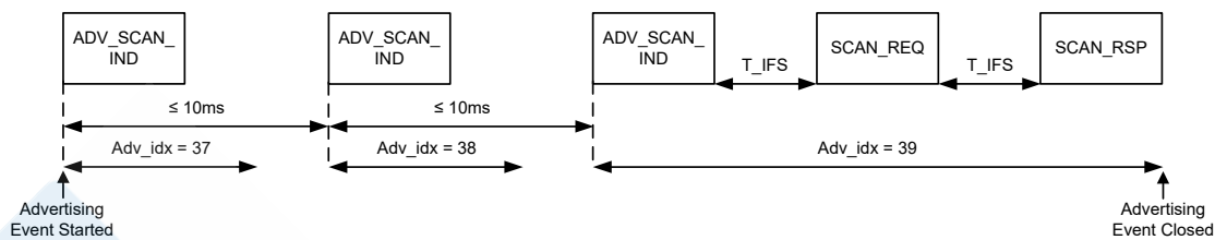
Scannable Event with SCAN_REQ and SCAN_RSP PDUs at the End of Event
