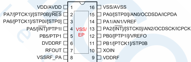
BC66F2123/BC66V2123 16 NSOP-EP-A
