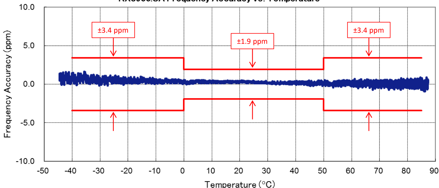
RX8900:UA Frequency Accuracy vs. Temperature
