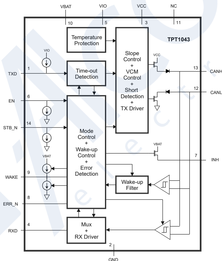
Figure 6. Functional Block Diagram
