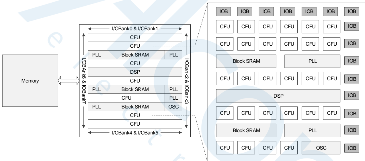
Figure 3-1 Architecture Diagram
