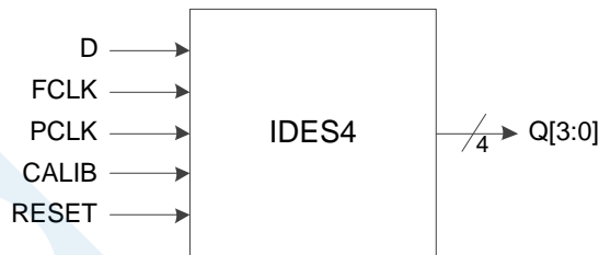
Figure 3-15 I/O Logic in IDES4 Mode
