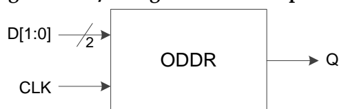
Figure 3-14 I/O Logic in DDR Output Mode
