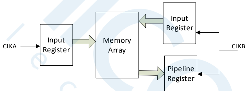
Figure 3-31 Read/Write Clock Mode
