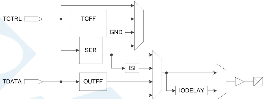
Figure 3-6 I/O Logic Input
