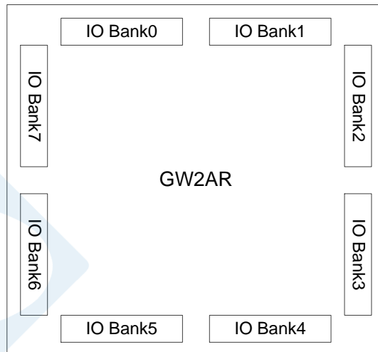
Figure 3-5 GW2AR I/O Bank Distribution
