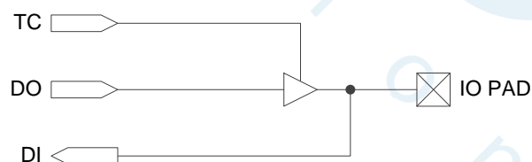
Figure 3-11 I/O Logic in Basic Mode
