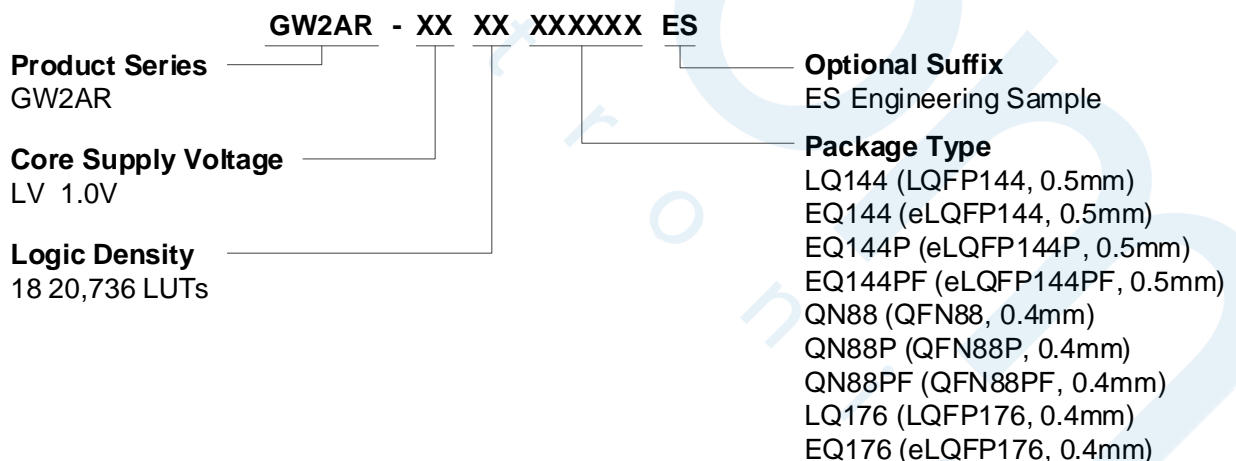
Figure 5-1 Part Naming of Devices with SDRAM Embedded-ES
