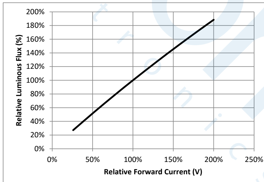
Figure 2: Relative Luminous Flux vs. Relative Forward Current, T_c=25^\circ\text{C}
