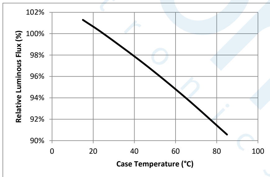
Figure 4: Relative Luminous Flux vs. Case Temperature For All Lengths, T_c=25^\circ\text{C}
