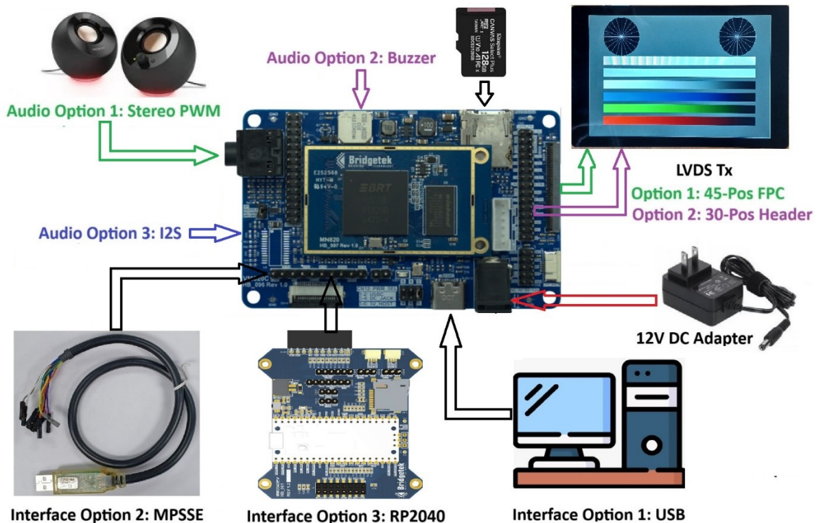
Figure 13 - MN820 Setup
