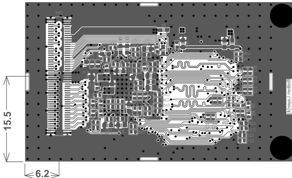
Figure 15 - MN820 PCBA Dimensions (Bottom View)
