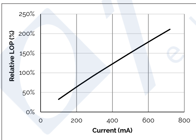
Figure 5: V6B Typical Relative Flux vs. Current
