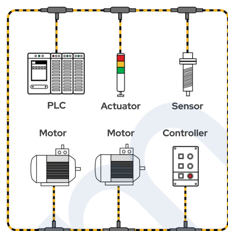
Ring Topology
