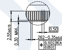
DETAIL E SCALE 2:1
